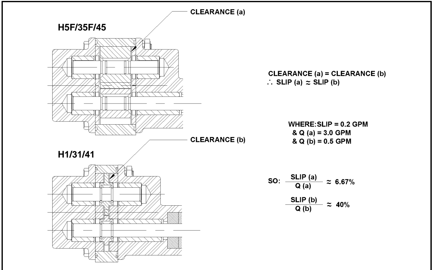
Diagram: Slip of Models H1/31/41 vs. Models H5F/35F/45
