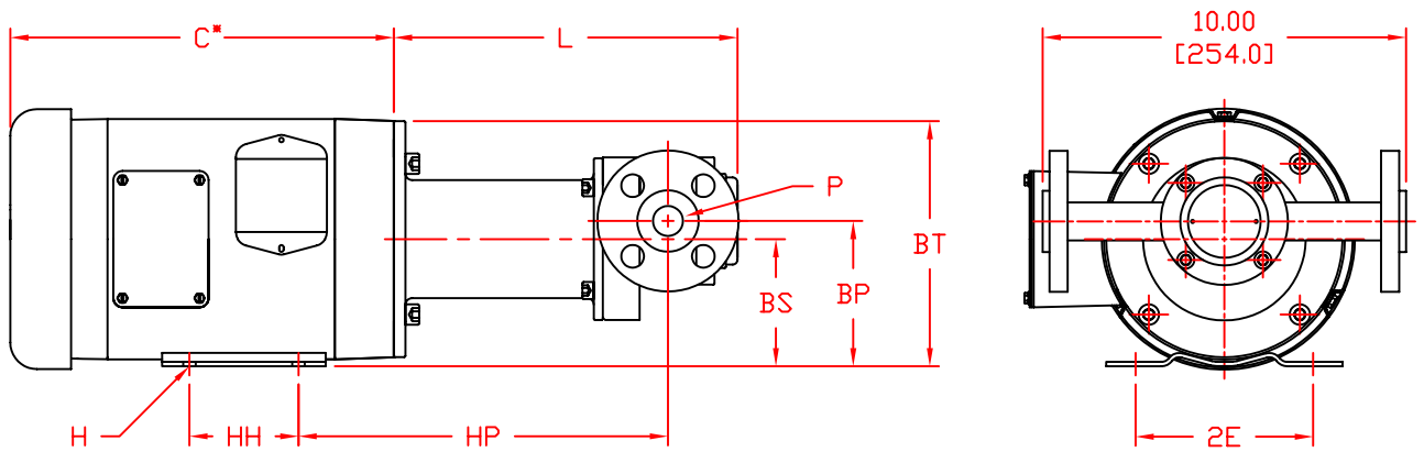
DIMENSIONAL DATA - NOT DEPENDENT ON MOTOR
