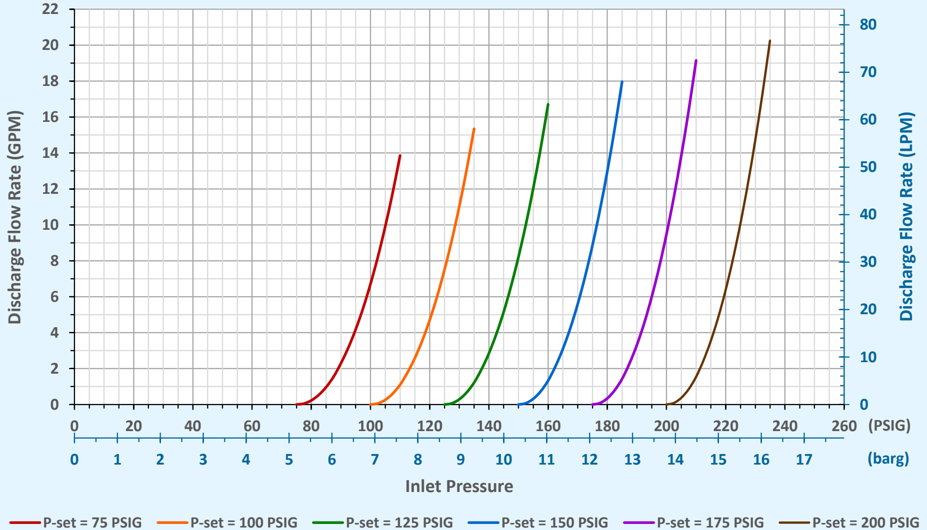
Models RV1000-HP & RV1001-HP Performance Curves: Discharge Flow Rate ( Q_d ) vs. Inlet Pressure ( P_{in} ) ( 75 \leq P_{set} \leq 200 ) Test Conditions: Water @ 70°F; discharge to atmosphere (0 PSIG)
