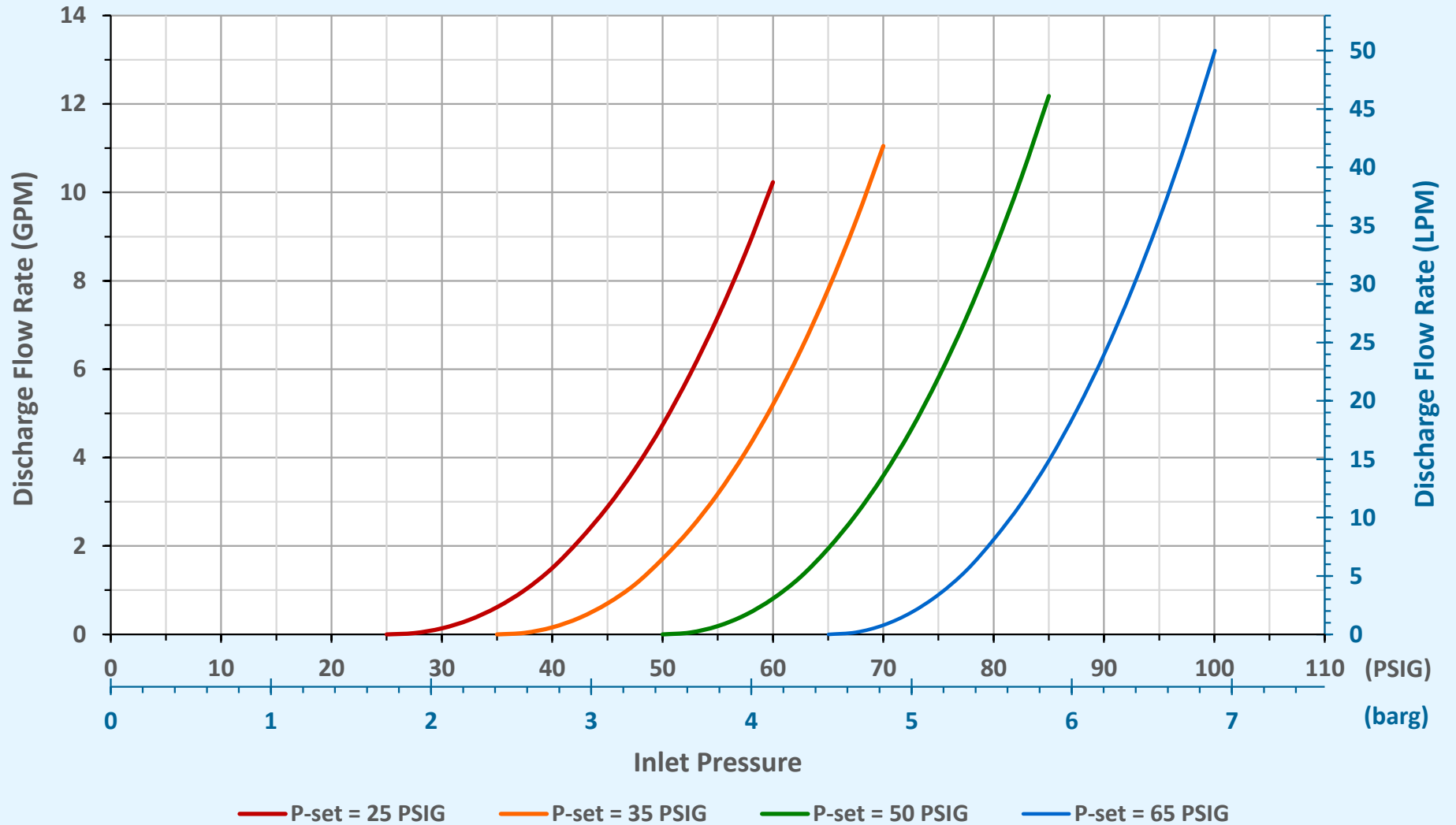
Models RV1000-LP & RV1001-LP Performance Curves: Discharge Flow Rate ( Q_d ) vs. Inlet Pressure ( P_{in} ) ( 25 \leq P_{set} \leq 65 ) Test Conditions: Water @ 70°F; discharge to atmosphere (0 PSIG)
