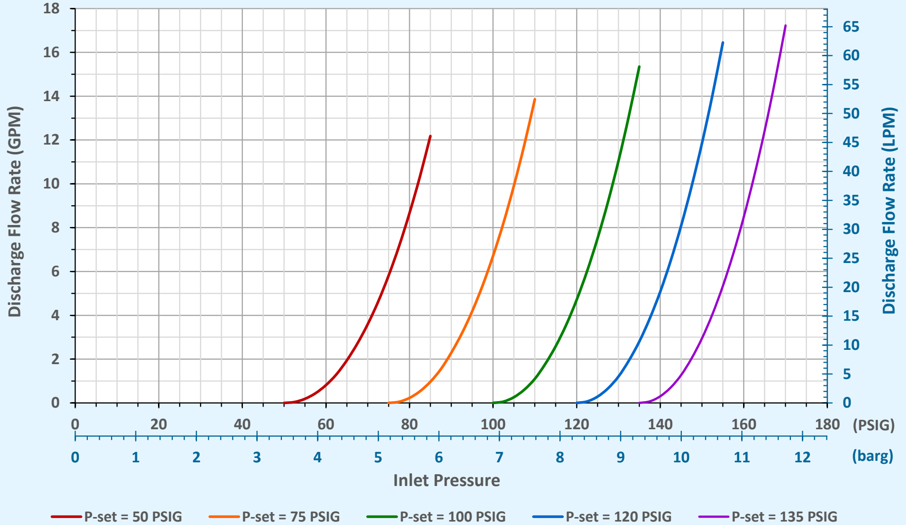
Models RV1000 & RV1001 Performance Curves: Discharge Flow Rate ( Q_d ) vs. Inlet Pressure ( P_{in} ) ( 50 \leq P_{set} \leq 135 ) Test Conditions: Water @ 70°F; discharge to atmosphere (0 PSIG)
