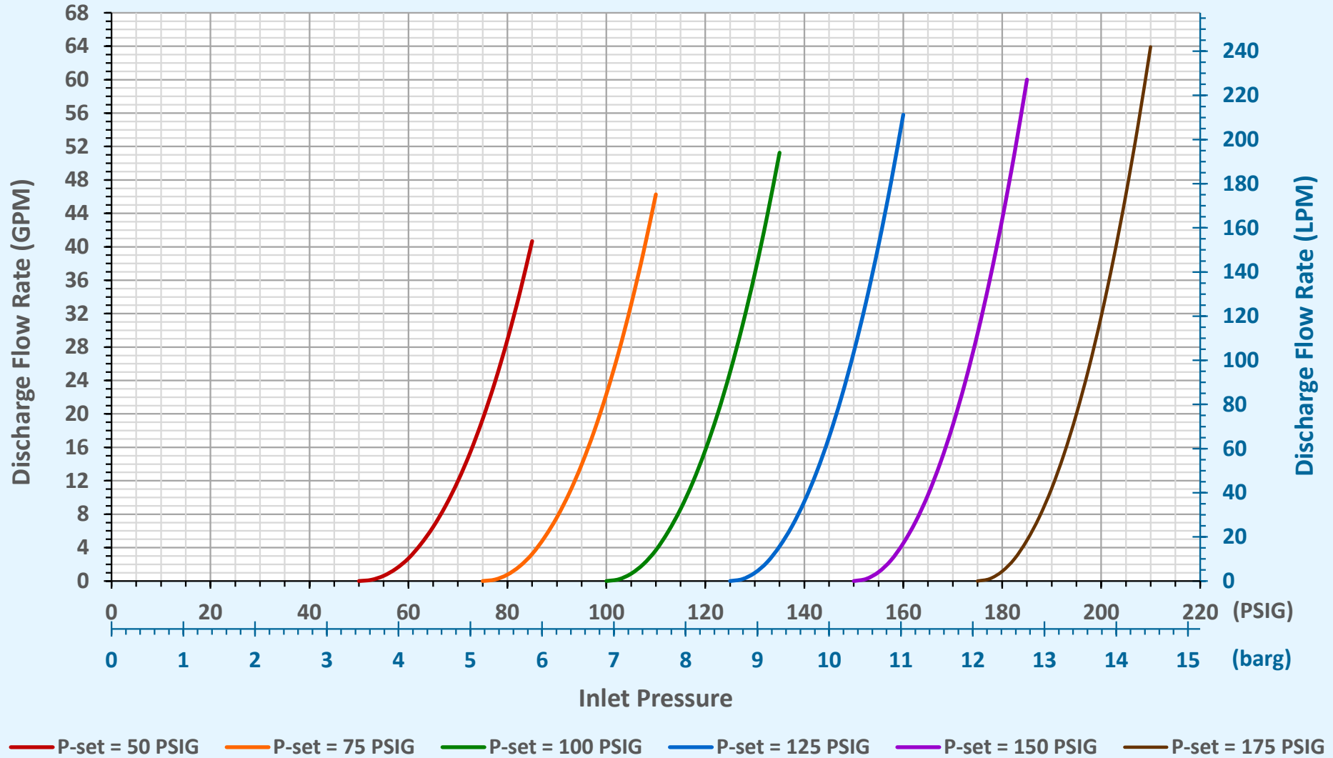
Models RV2000 & RV2001 Performance Curves: Discharge Flow Rate ( Q_d ) vs. Inlet Pressure ( P_{in} ) ( 50 \leq P_{set} \leq 175 ) Test Conditions: Water @ 70°F; discharge to atmosphere (0 PSIG)
